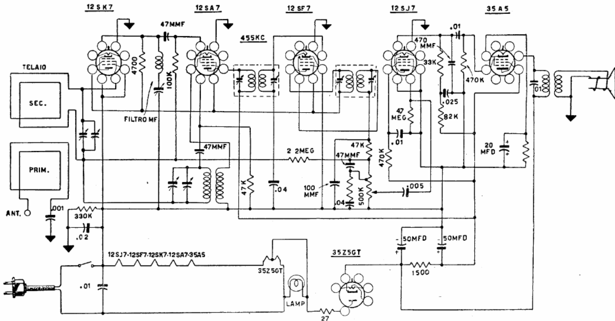
Fig. 8.17. - Supereterodina Westinghouse mod. H 125/126.
